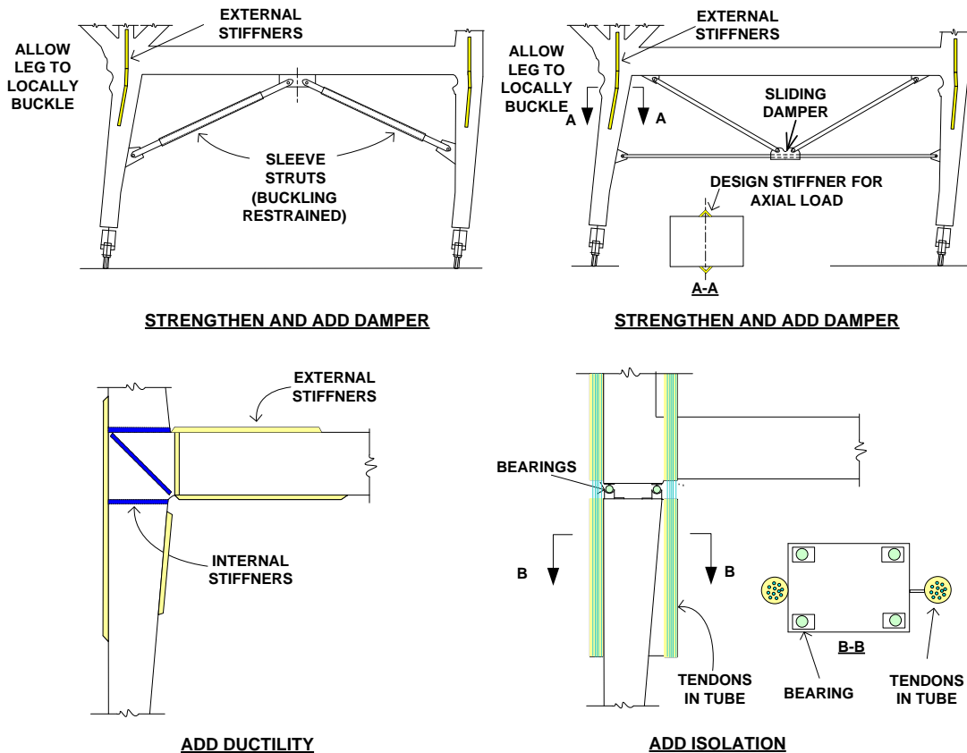
Figure 8. Retrofit concepts
